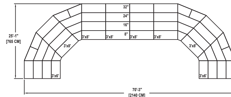
SEMICIRCLE SHAPE
