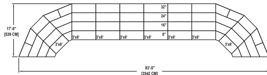
ARC SHAPE
